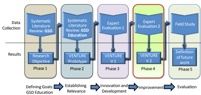
Figure 4. Research method.
